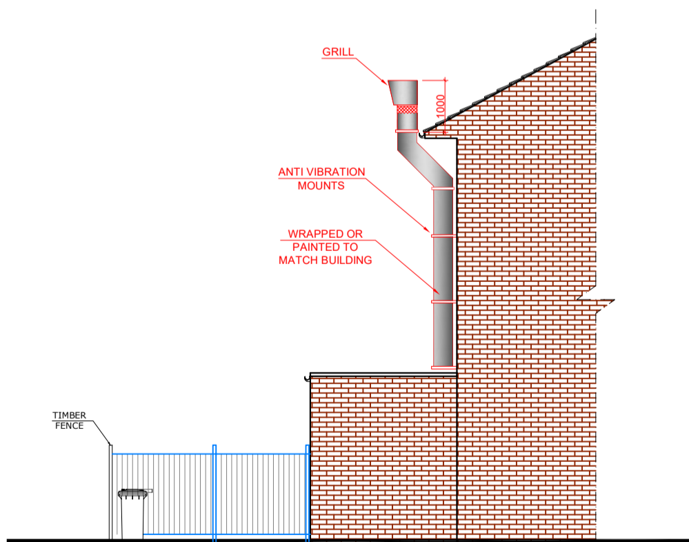
PROPOSED SIDE ELEVATION SCALE: 1/100 @A3
